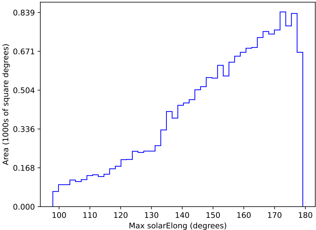
too_elab_r32_d3_giz_v3.4_10yrs WFD u band: Max solarElong
