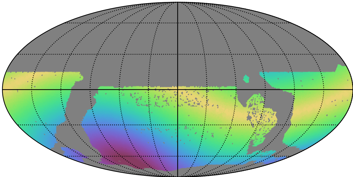
too_elab_r32_d3_giz_v3.4_10yrs WFD r band: Max solarElong
