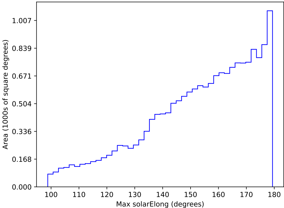
too_elab_r32_d3_giz_v3.4_10yrs WFD r band: Max solarElong
