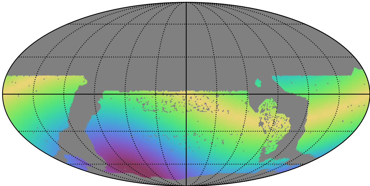
too_elab_r32_d3_giz_v3.4_10yrs WFD i band: Max solarElong
