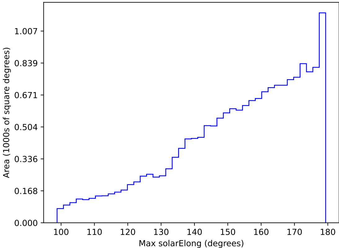
too_elab_r32_d3_giz_v3.4_10yrs WFD i band: Max solarElong
