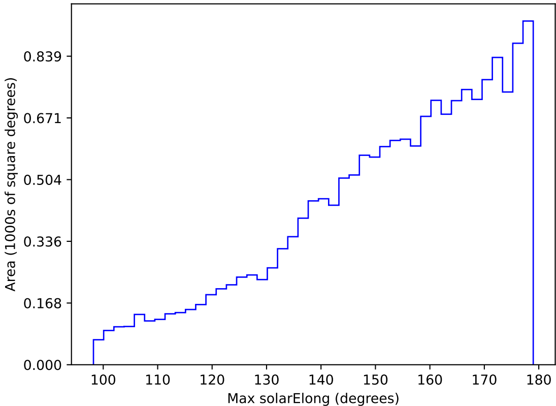
too_elab_r32_d3_giz_v3.4_10yrs WFD g band: Max solarElong
