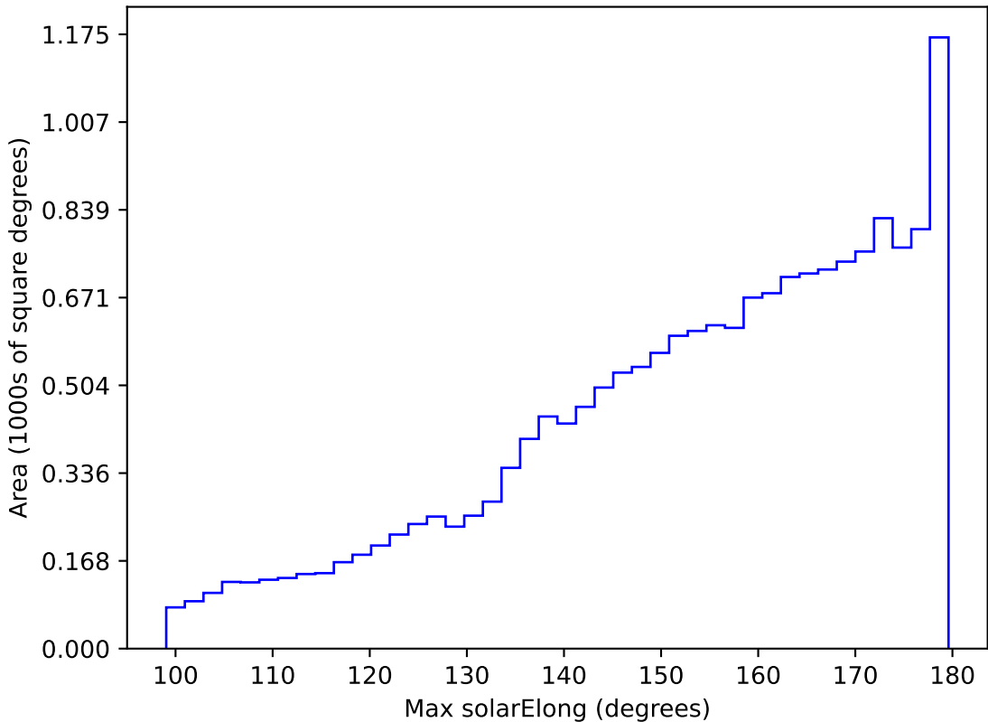
too_elab_r32_d3_giz_v3.4_10yrs WFD all bands: Max solarElong
