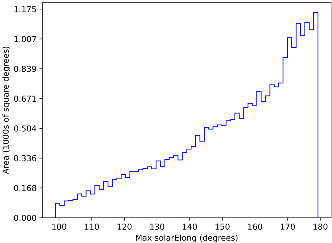
too_elab_r32_d3_giz_v3.4_10yrs All sky z band: Max solarElong
