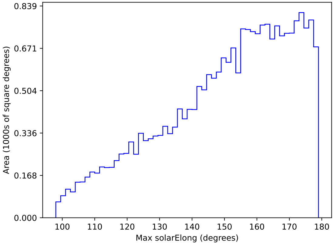
too_elab_r32_d3_giz_v3.4_10yrs All sky u band: Max solarElong
