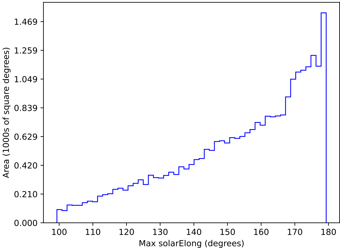
too_elab_r32_d3_giz_v3.4_10yrs All sky r band: Max solarElong
