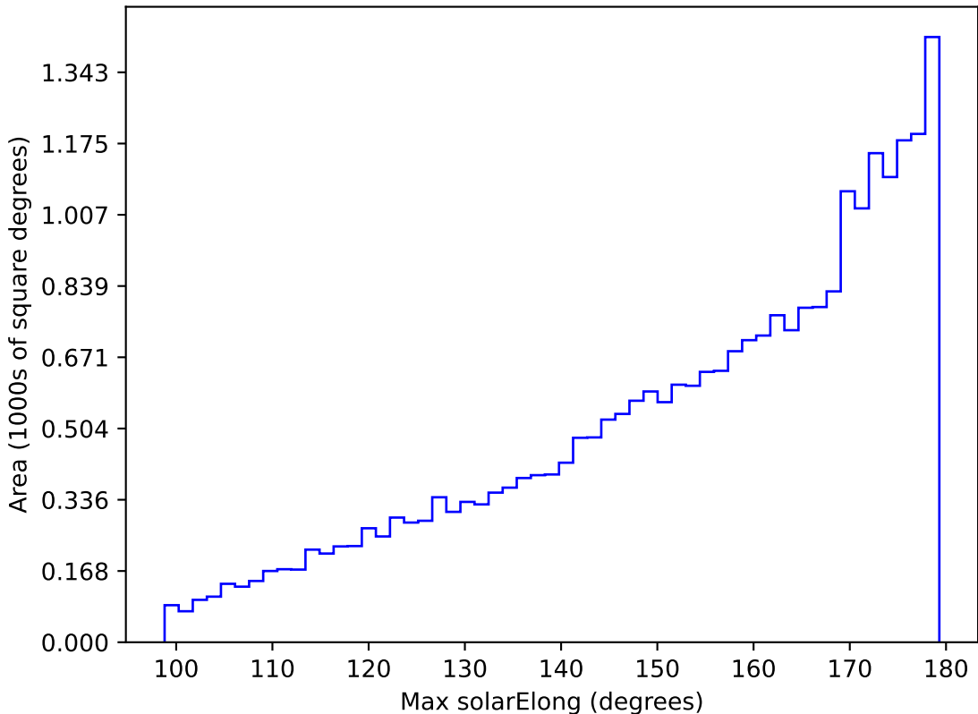
too_elab_r32_d3_giz_v3.4_10yrs All sky i band: Max solarElong
