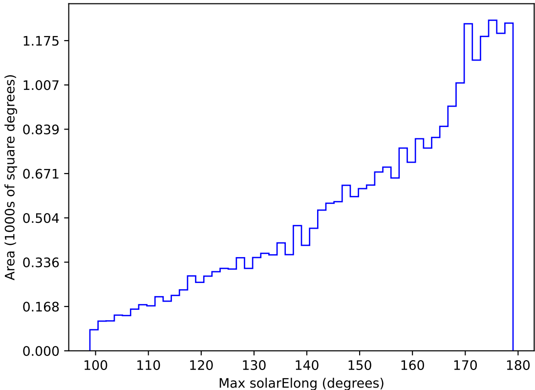
too_elab_r32_d3_giz_v3.4_10yrs All sky g band: Max solarElong
