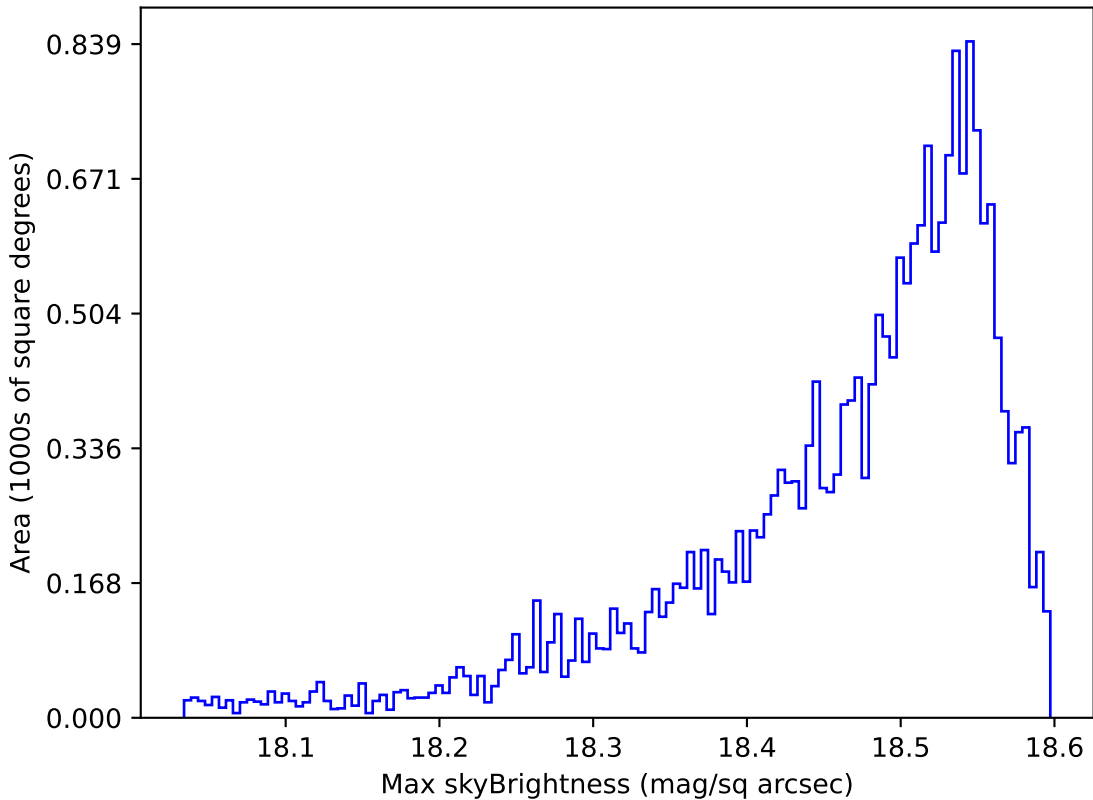
too_elab_r32_d3_giz_v3.4_10yrs Yr 1 y band: Max skyBrightness
