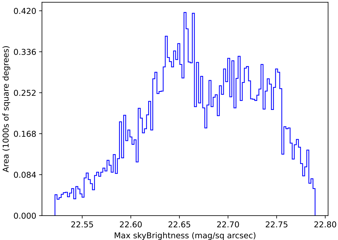
too_elab_r32_d3_giz_v3.4_10yrs Yr 1 u band: Max skyBrightness
