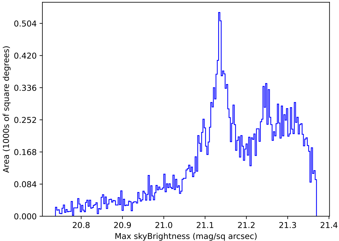
too_elab_r32_d3_giz_v3.4_10yrs Yr 1 r band: Max skyBrightness
