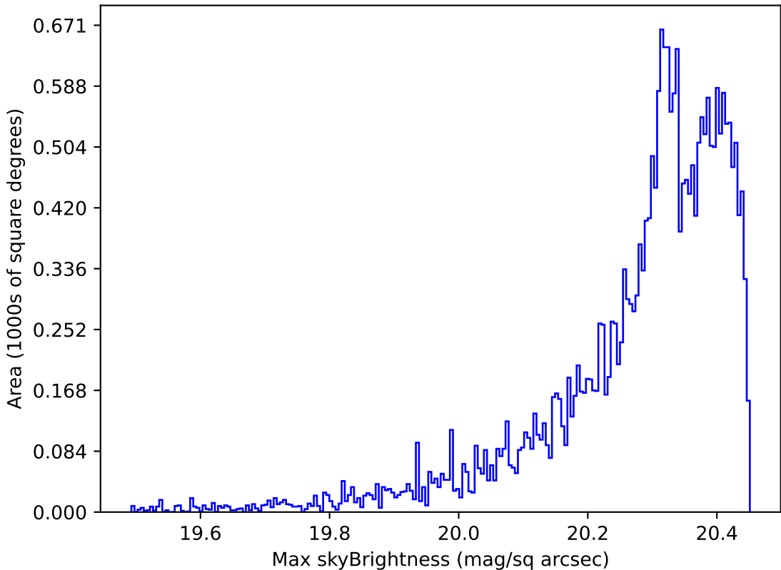
too_elab_r32_d3_giz_v3.4_10yrs Yr 1 i band: Max skyBrightness
