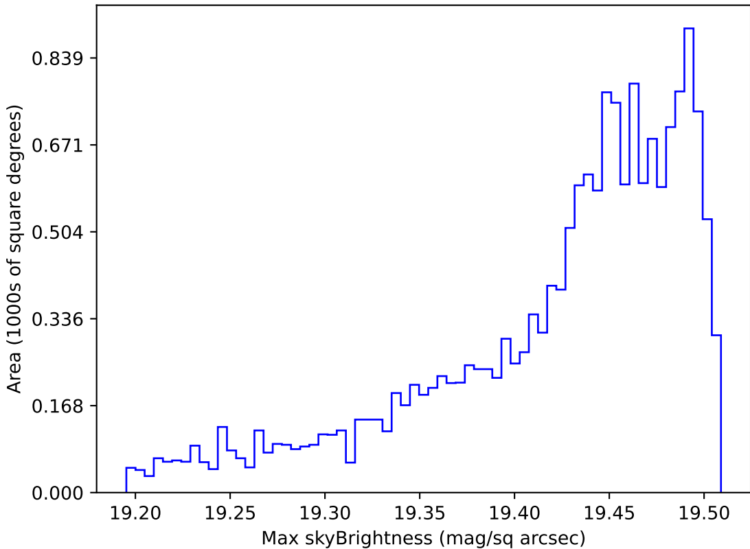
too_elab_r32_d3_giz_v3.4_10yrs WFD z band: Max skyBrightness
