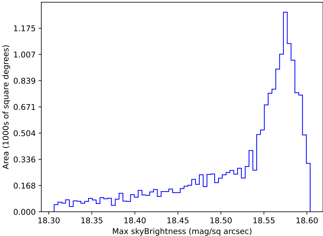
too_elab_r32_d3_giz_v3.4_10yrs WFD y band: Max skyBrightness
