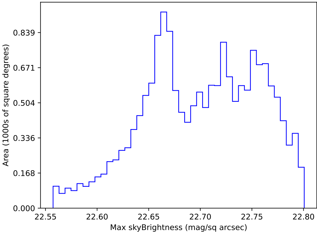
too_elab_r32_d3_giz_v3.4_10yrs WFD u band: Max skyBrightness
