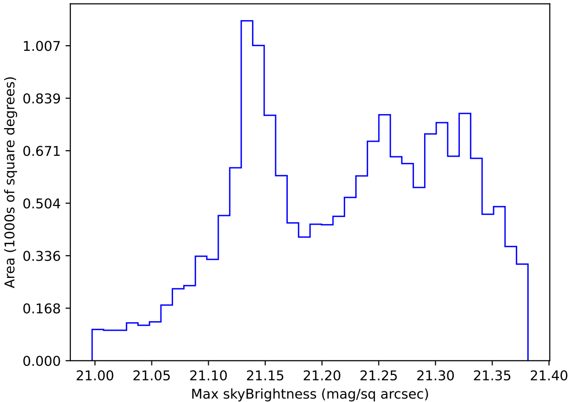
too_elab_r32_d3_giz_v3.4_10yrs WFD r band: Max skyBrightness
