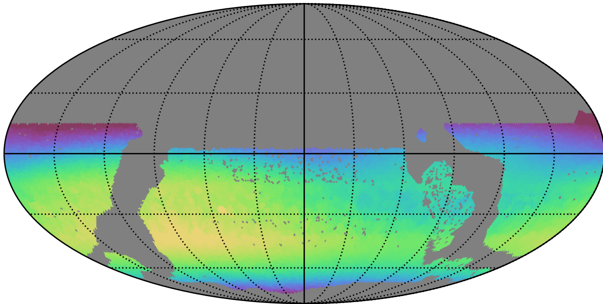
too_elab_r32_d3_giz_v3.4_10yrs WFD i band: Max skyBrightness
