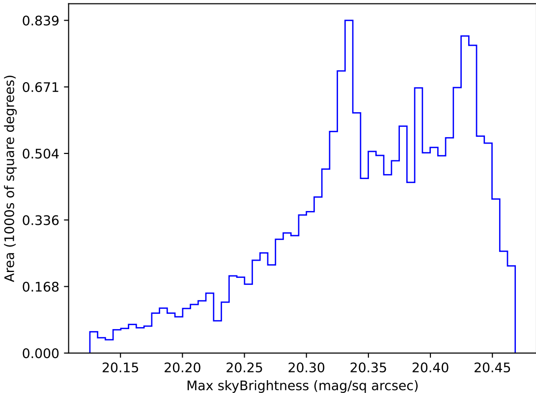
too_elab_r32_d3_giz_v3.4_10yrs WFD i band: Max skyBrightness
