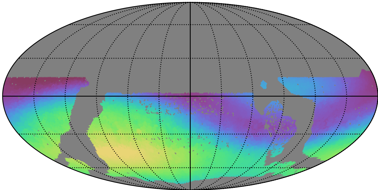
too_elab_r32_d3_giz_v3.4_10yrs WFD g band: Max skyBrightness
