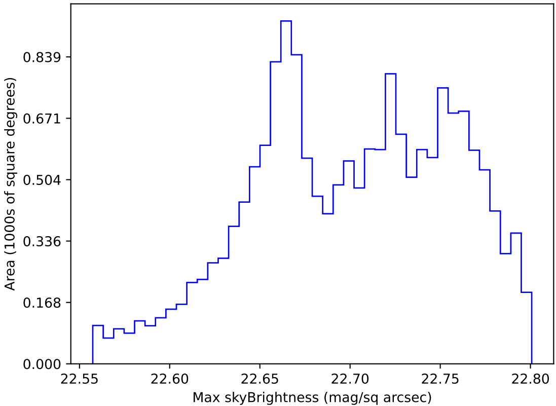
too_elab_r32_d3_giz_v3.4_10yrs WFD all bands: Max skyBrightness
