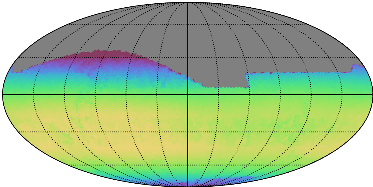
too_elab_r32_d3_giz_v3.4_10yrs All sky z band: Max skyBrightness
