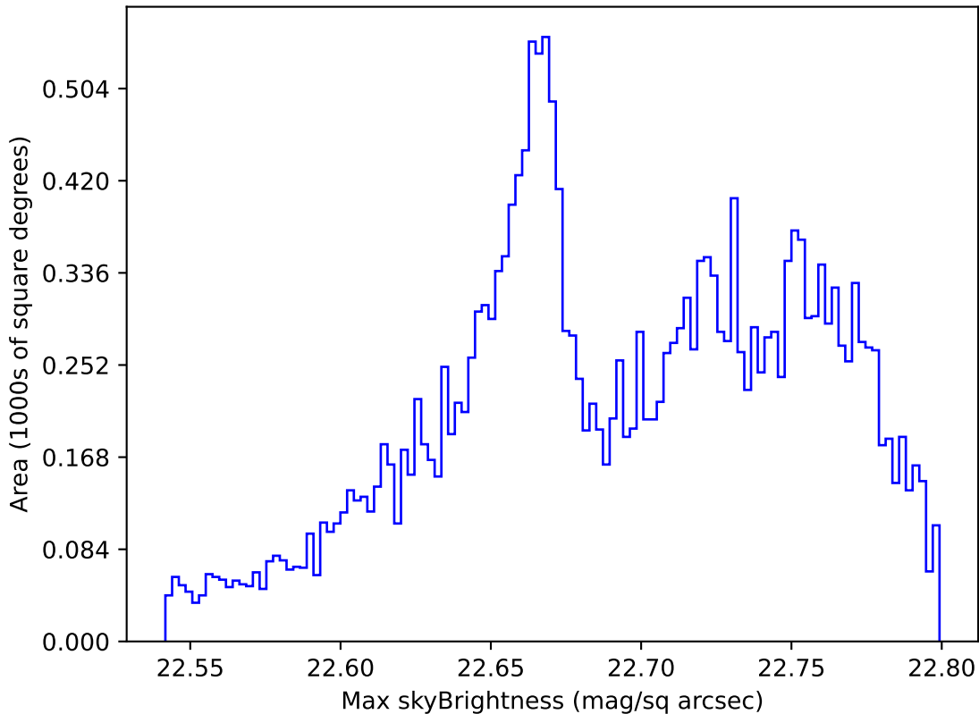
too_elab_r32_d3_giz_v3.4_10yrs All sky u band: Max skyBrightness
