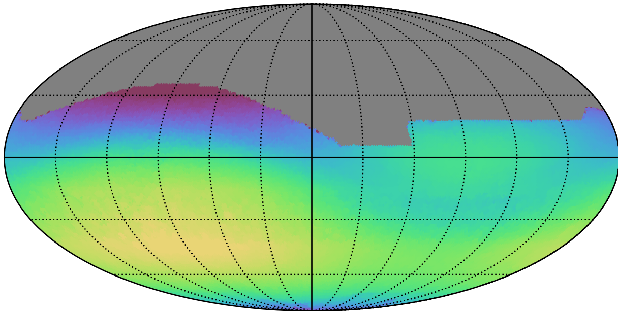
too_elab_r32_d3_giz_v3.4_10yrs All sky r band: Max skyBrightness
