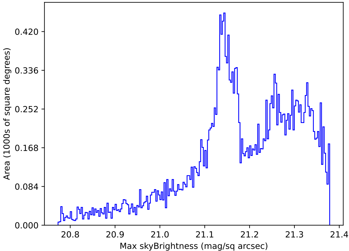
too_elab_r32_d3_giz_v3.4_10yrs All sky r band: Max skyBrightness
