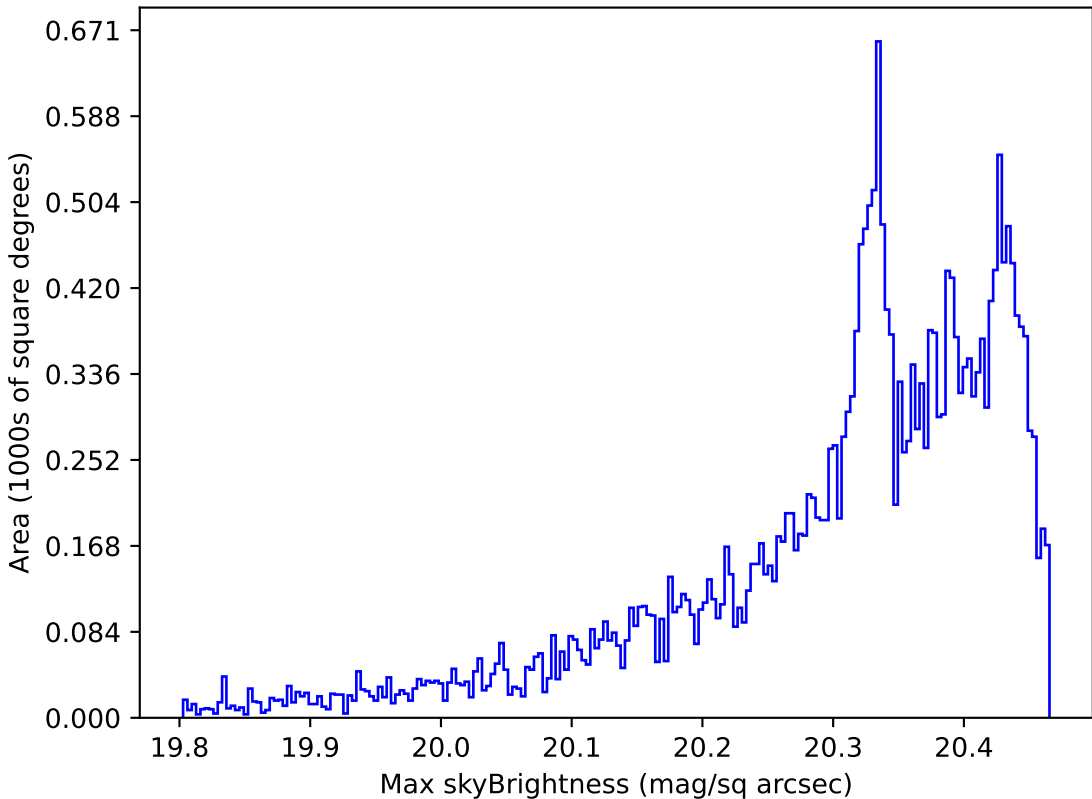
too_elab_r32_d3_giz_v3.4_10yrs All sky i band: Max skyBrightness
