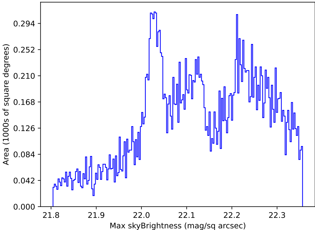
too_elab_r32_d3_giz_v3.4_10yrs All sky g band: Max skyBrightness
