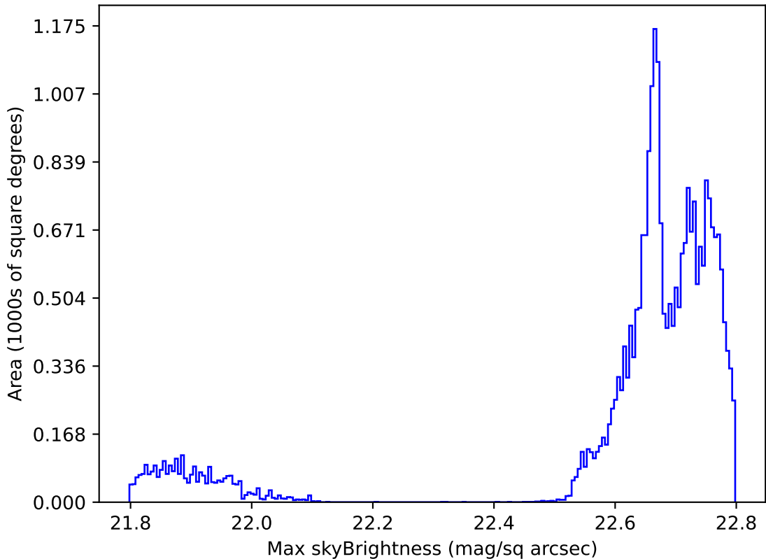
too_elab_r32_d3_giz_v3.4_10yrs All sky all bands: Max skyBrightness
