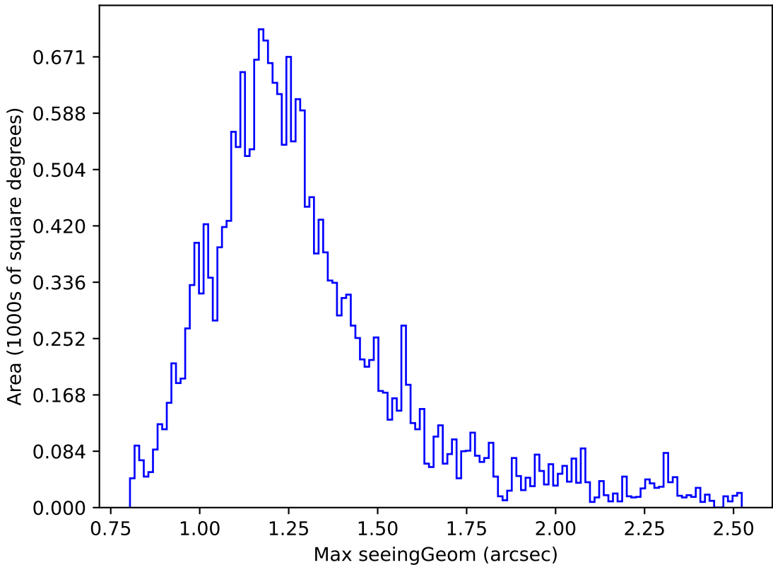
too_elab_r32_d3_giz_v3.4_10yrs Yr 1 y band: Max seeingGeom
