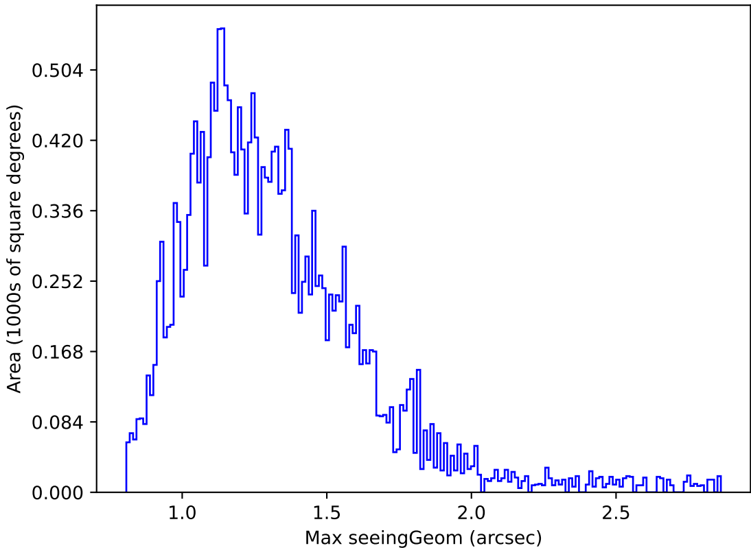
too_elab_r32_d3_giz_v3.4_10yrs Yr 1 u band: Max seeingGeom
