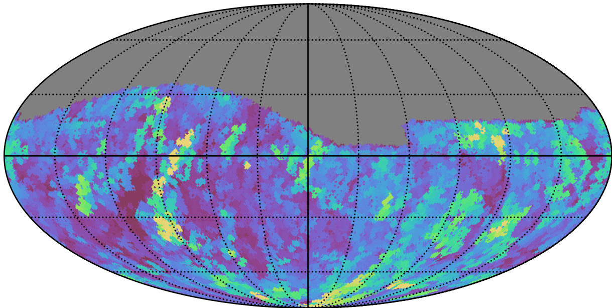
too_elab_r32_d3_giz_v3.4_10yrs Yr 1 r band: Max seeingGeom
