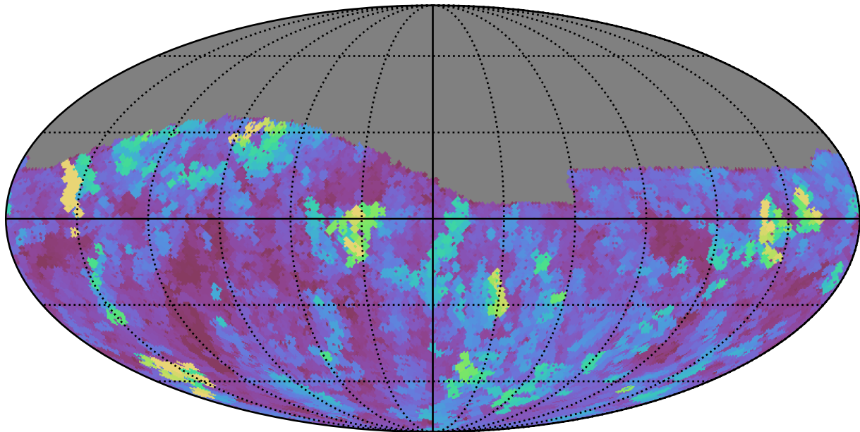
too_elab_r32_d3_giz_v3.4_10yrs Yr 1 i band: Max seeingGeom
