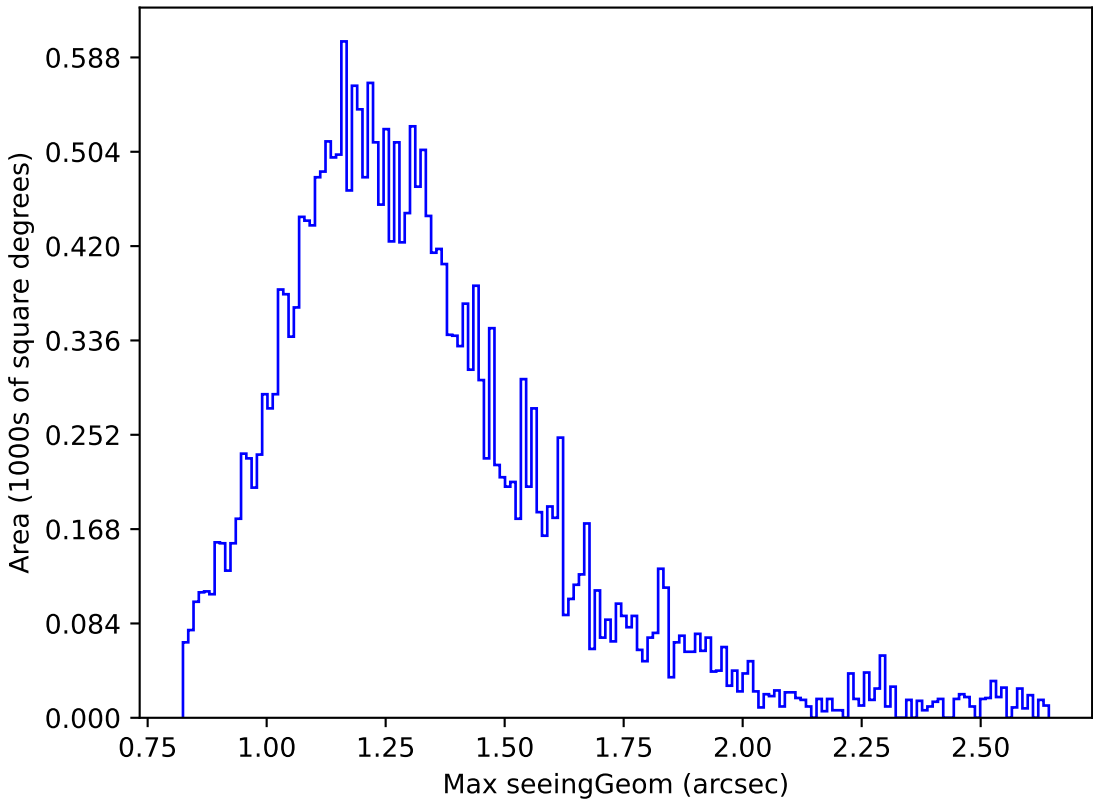
too_elab_r32_d3_giz_v3.4_10yrs Yr 1 i band: Max seeingGeom
