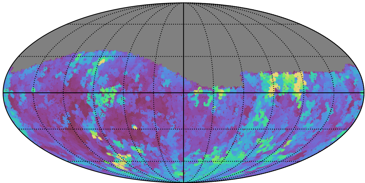
too_elab_r32_d3_giz_v3.4_10yrs Yr 1 g band: Max seeingGeom
