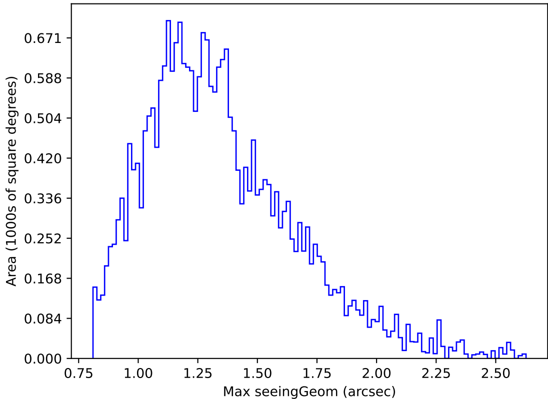
too_elab_r32_d3_giz_v3.4_10yrs Yr 1 g band: Max seeingGeom
