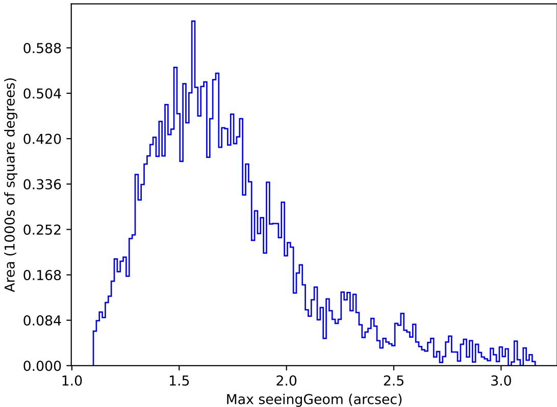
too_elab_r32_d3_giz_v3.4_10yrs Yr 1 all bands: Max seeingGeom
