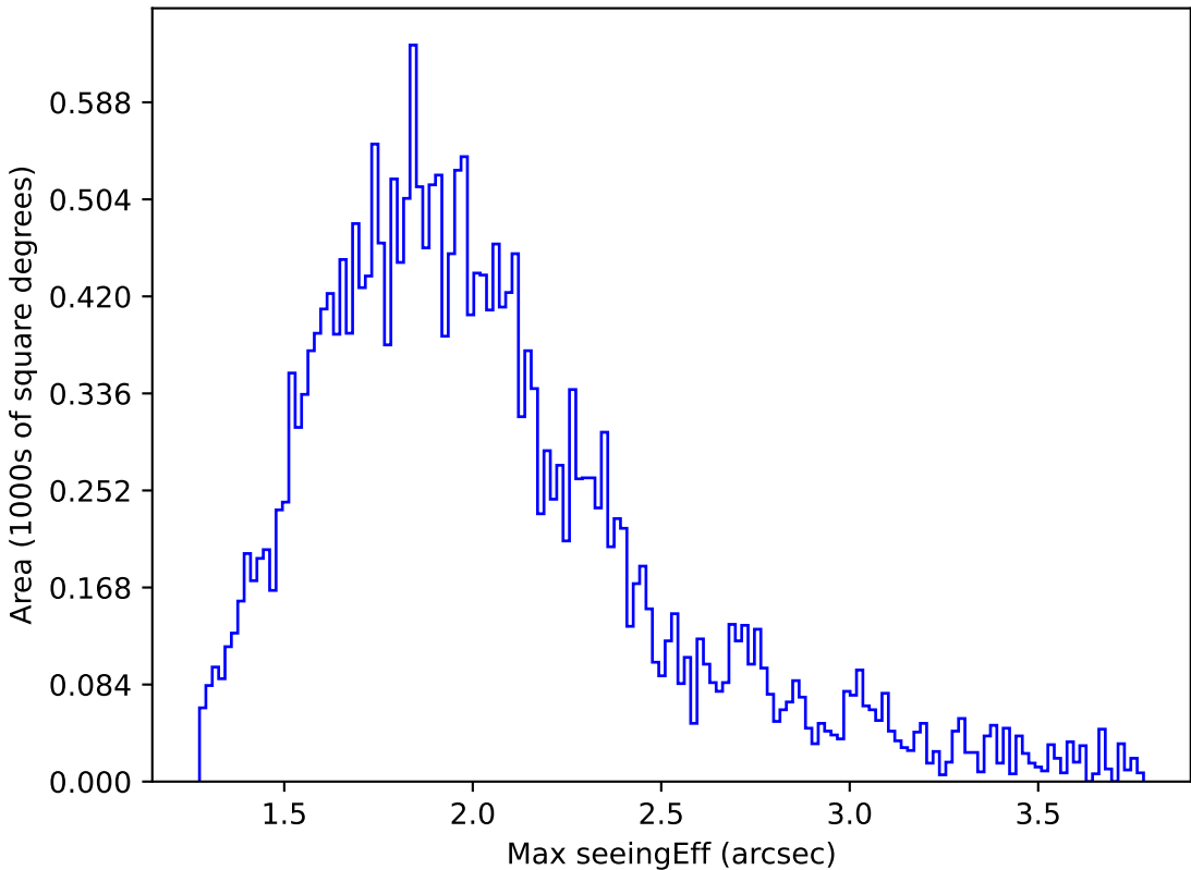
too_elab_r32_d3_giz_v3.4_10yrs Yr 1 all bands: Max seeingEff
