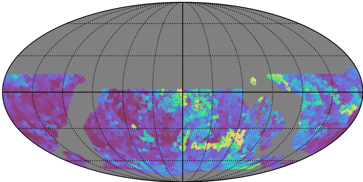
too_elab_r32_d3_giz_v3.4_10yrs WFD y band: Max seeingEff
