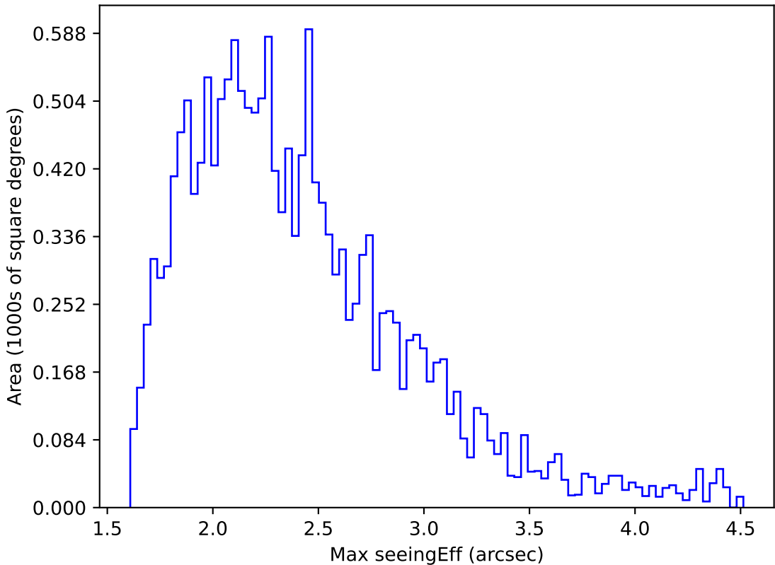
too_elab_r32_d3_giz_v3.4_10yrs WFD y band: Max seeingEff
