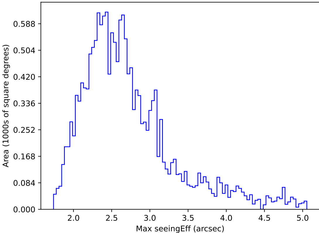
too_elab_r32_d3_giz_v3.4_10yrs WFD i band: Max seeingEff
