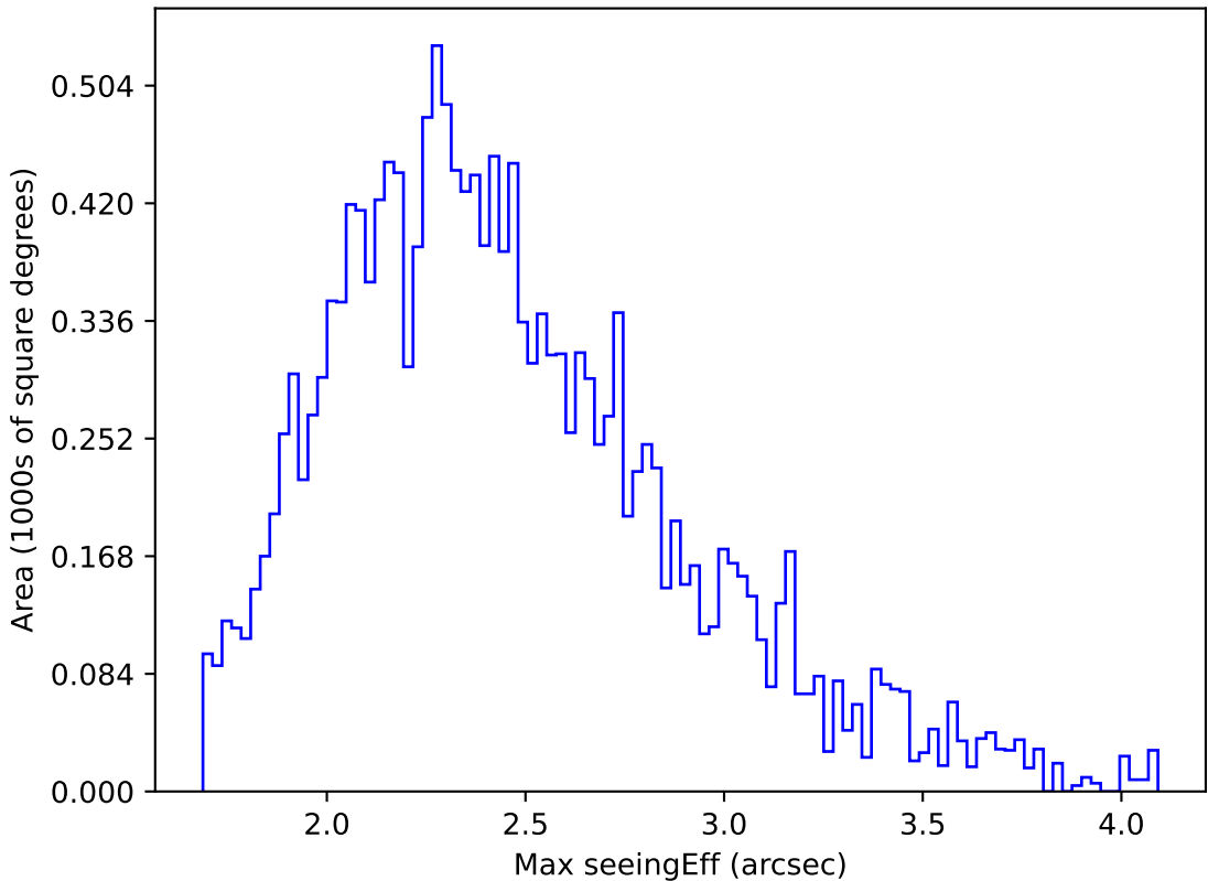
too_elab_r32_d3_giz_v3.4_10yrs WFD g band: Max seeingEff
