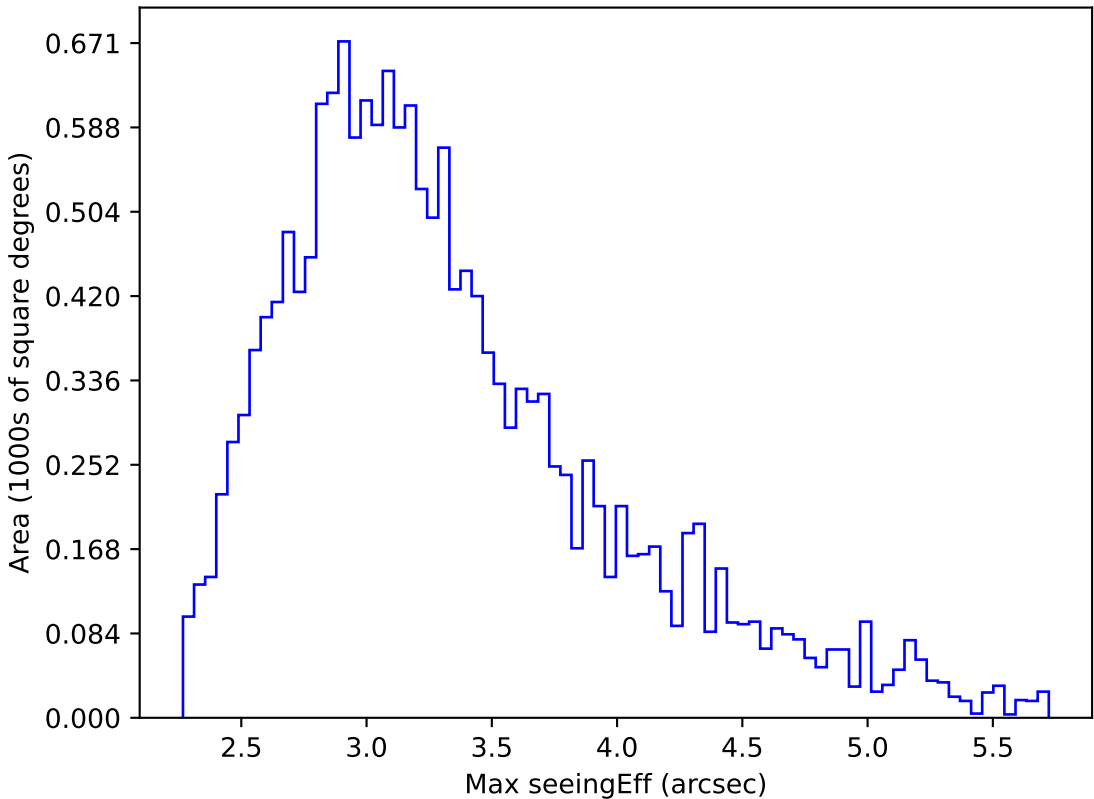
too_elab_r32_d3_giz_v3.4_10yrs WFD all bands: Max seeingEff
