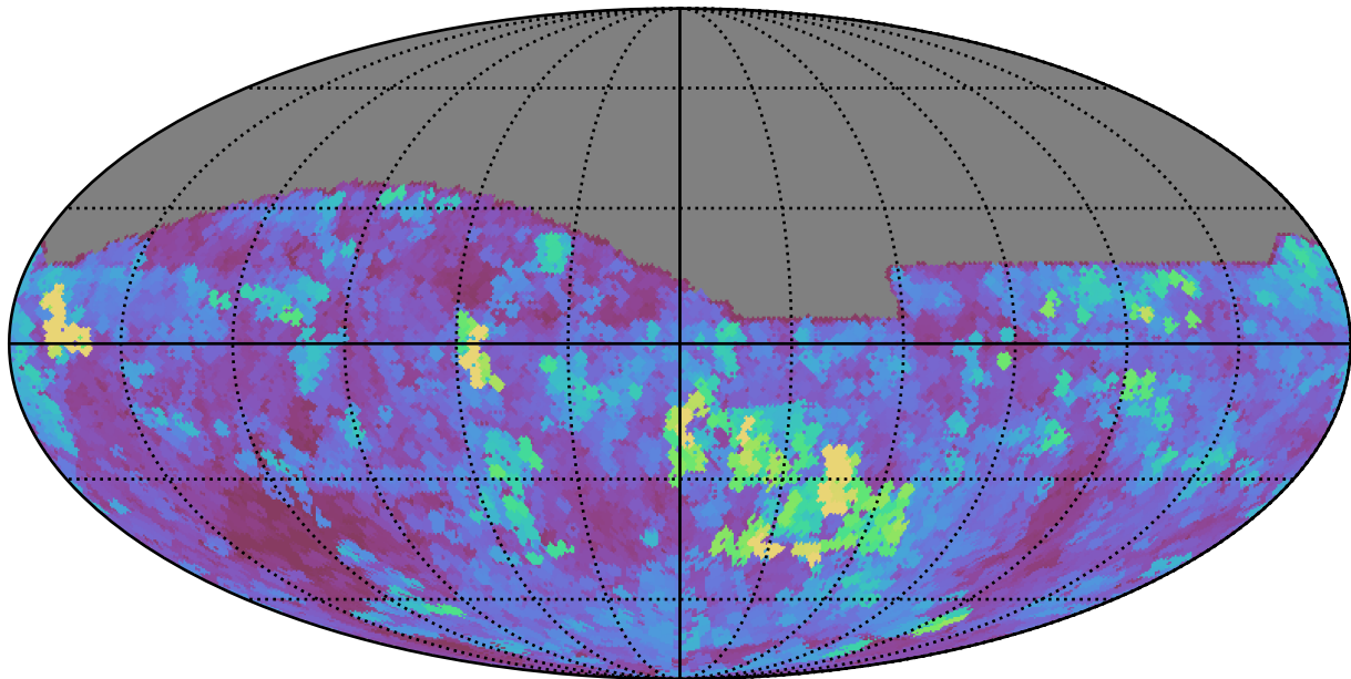
too_elab_r32_d3_giz_v3.4_10yrs All sky z band: Max seeingEff
