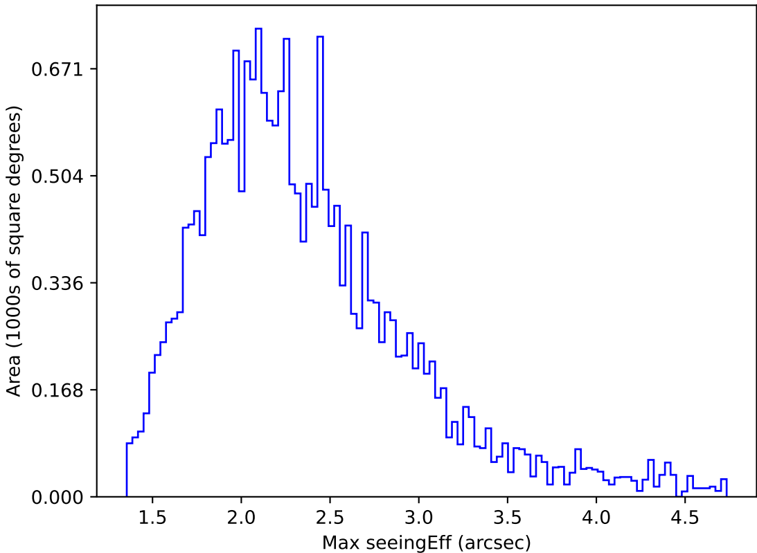
too_elab_r32_d3_giz_v3.4_10yrs All sky y band: Max seeingEff
