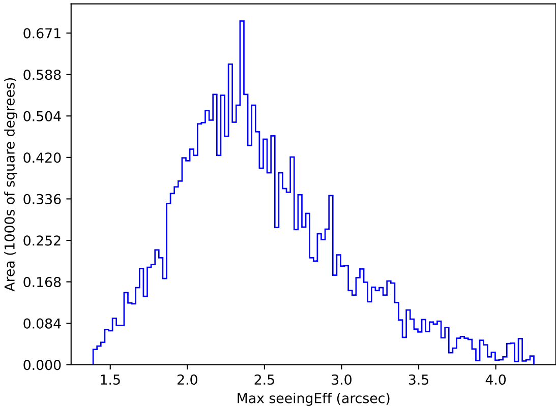
too_elab_r32_d3_giz_v3.4_10yrs All sky u band: Max seeingEff
