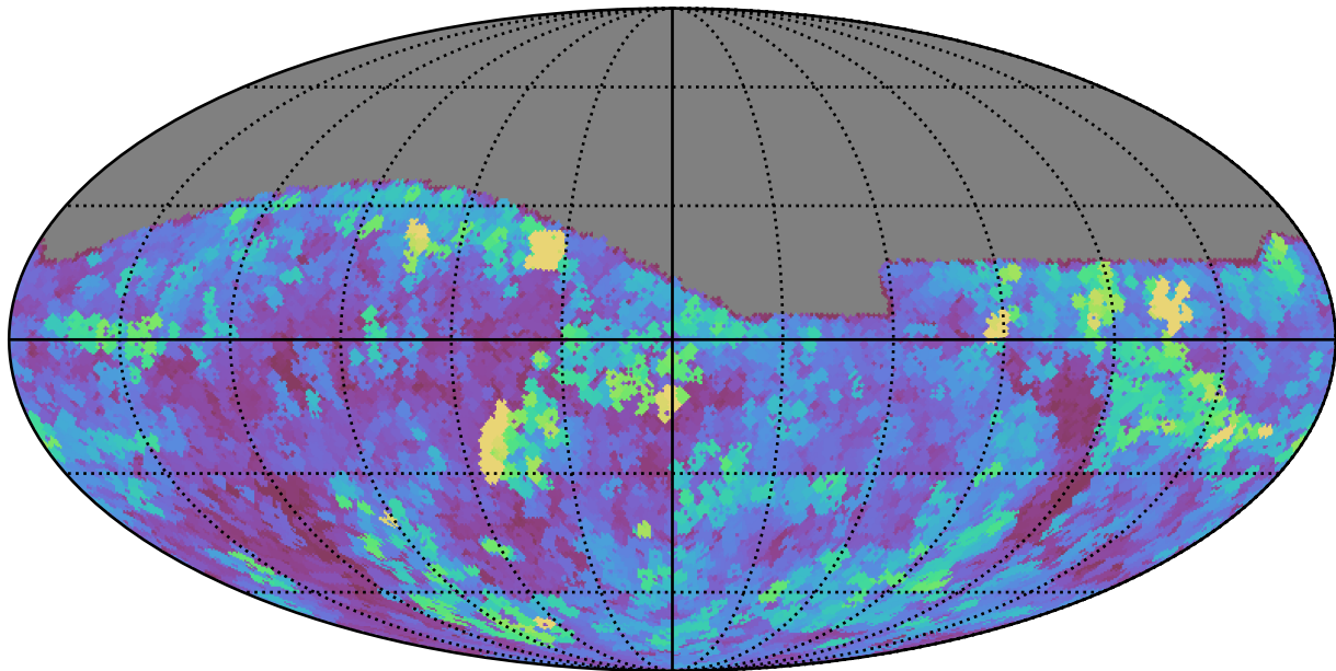
too_elab_r32_d3_giz_v3.4_10yrs All sky g band: Max seeingEff
