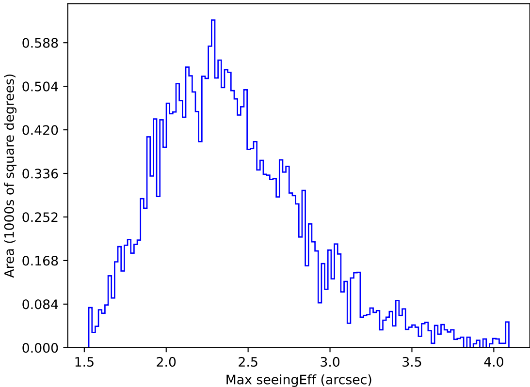
too_elab_r32_d3_giz_v3.4_10yrs All sky g band: Max seeingEff
